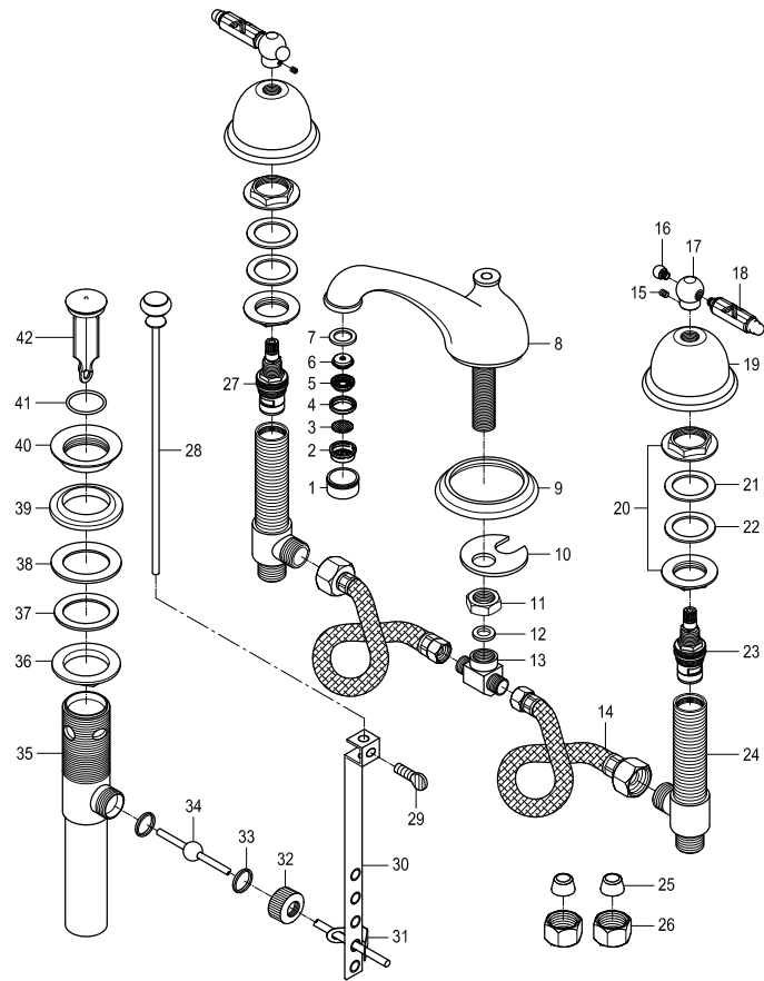
Cold Cartridge: KSRPL3000CC
